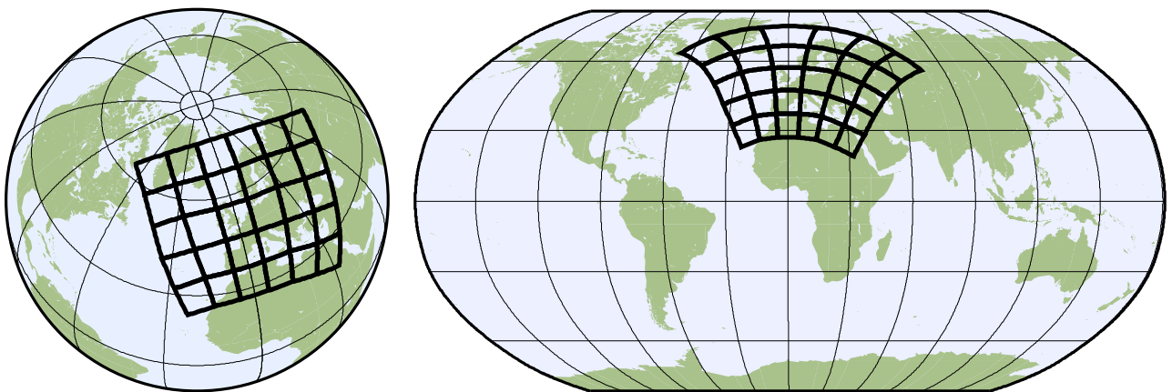
Figure A.1.: Orthographic and Robinson projection of the curvilinear grid
