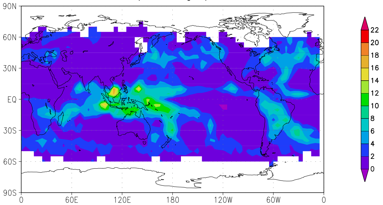
GPCP Precipitation 00Z01DEC1996 (mm d -1 ) (5° x 5° grid)
