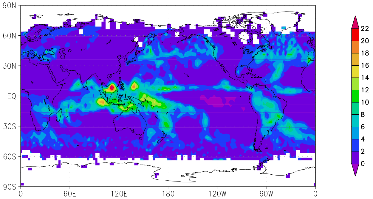
GPCP Precipitation 00Z01DEC1996 (mm d -1 ) (2.5° x 2.5° grid)
